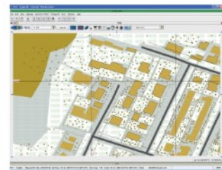
OneSAF
